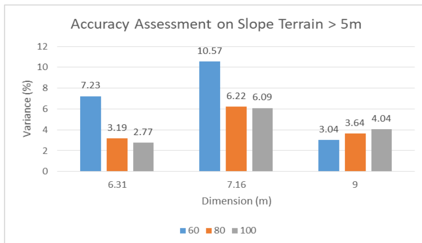
Fig. 8: Graph of Accuracy Assessment on Slope Surface more than 5m
