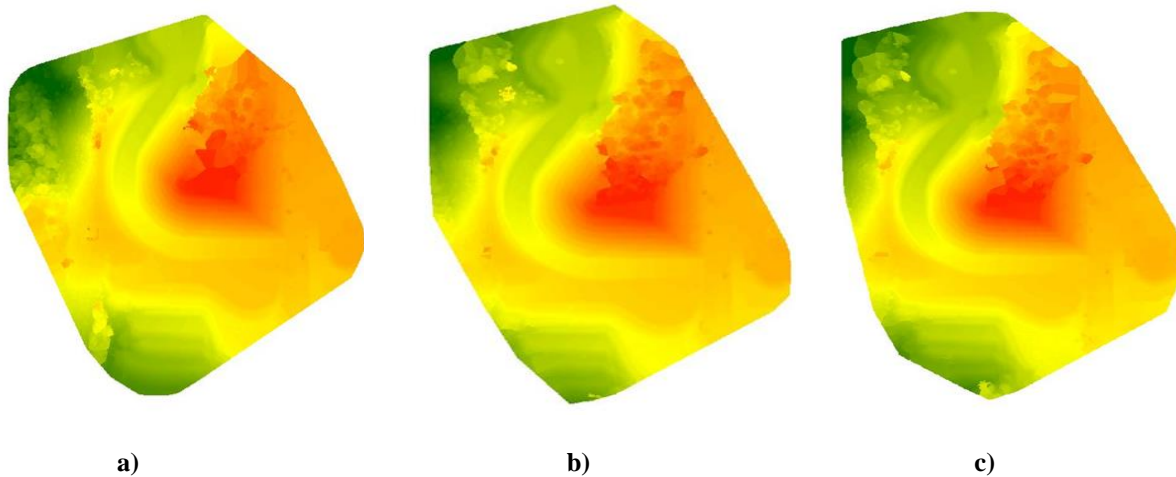
Fig. 3: Digital Surface Model (DSM) of Different Altitudes; a) 60m, b) 80m, c) 100m
