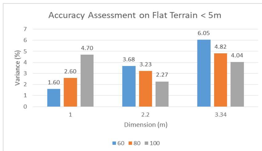
Fig. 6: Graph of Accuracy Assessment on Flat Terrain not more than 5m
