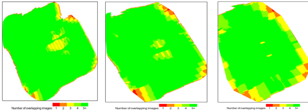
c) b) c) Fig. 5: Overlapping Images of Different Altitudes; a)60m, b)80m, c)100m
